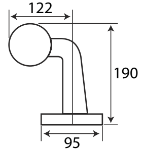
▪ universal LED marker lamp
