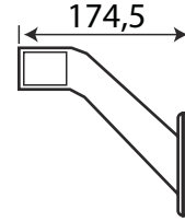
▪ universal LED marker lamp
